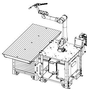
1-Sided Cobot Welding Table 72" x 36" Cobot Welding Table with Docking Station MSRP $9,800
