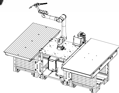
2-Sided Welding & Quick-Change Tables 72" x 36" Cobot Welding Table 72" x 36" Quick-Change Table with Docking Station MSRP $18,800
